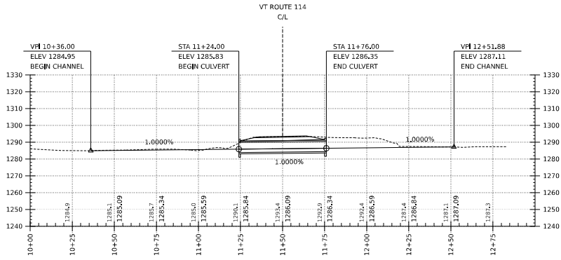
CHANNEL PROFILE
