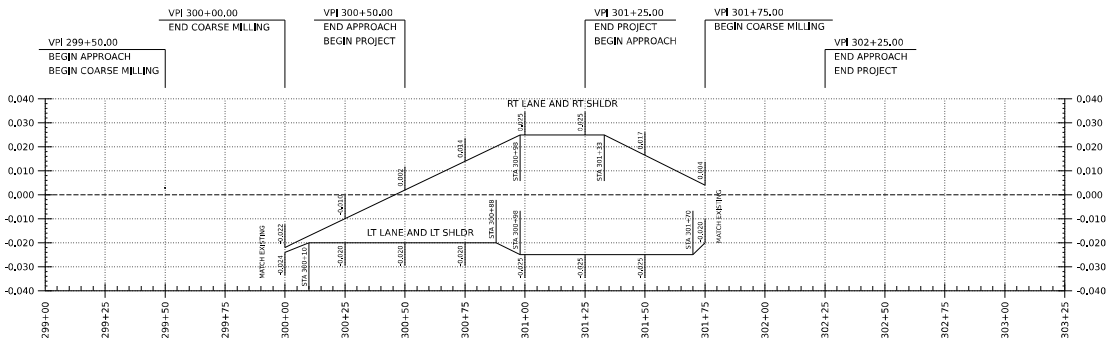
VT ROUTE 114 BANKING DIAGRAM
