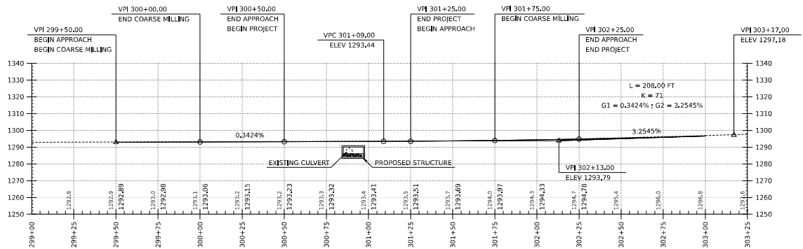
VT ROUTE 114 PROFILE
