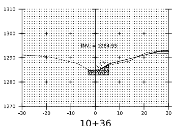
10+36 BEGIN CHANNEL
