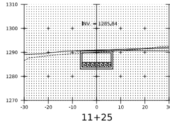
11+25
