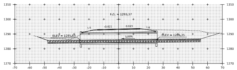
300+91 SKEWED 10° BRIDGE #43
