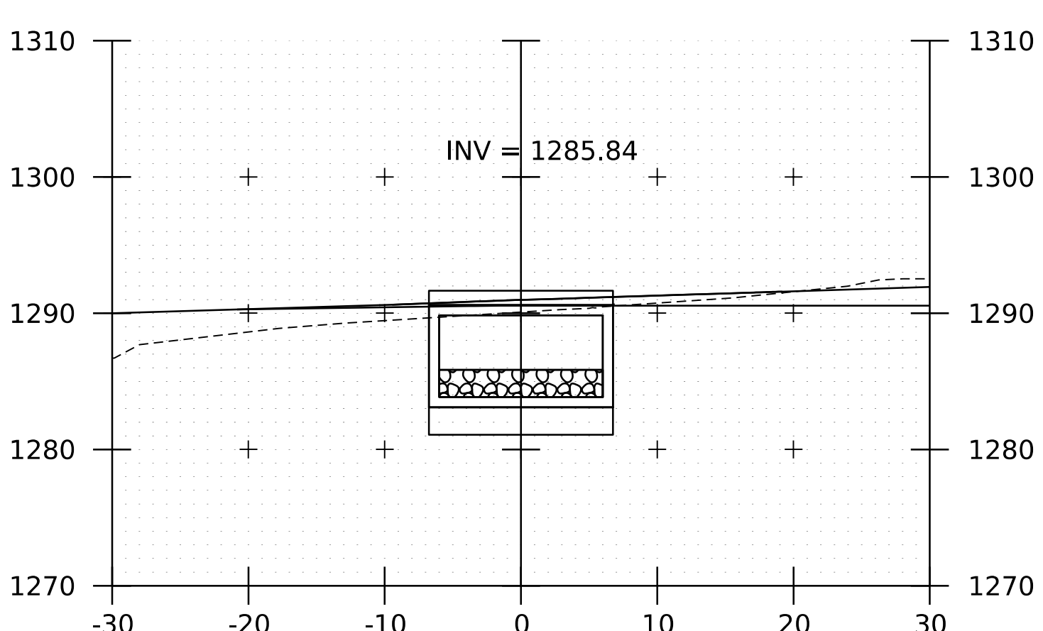
11+25
