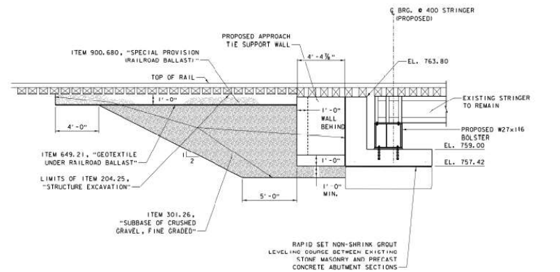
ABUTMENT 1 - PROPOSED SECTION (AT CL. 400 STRINGER) SCALE: \frac{3}{8}'' = 1'-0''
