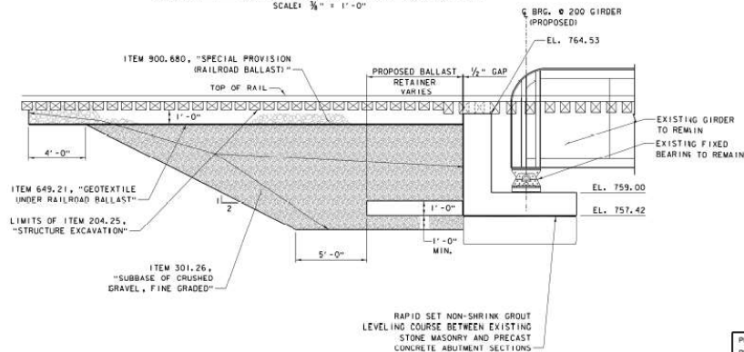
ABUTMENT 1 - PROPOSED SECTION (AT CL. 200 GIRDER) SCALE: \frac{3}{8}'' = 1'-0''
