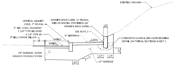
STOWE STREET RT NOT TO SCALE STA. 30+16 - 30+88 RT
