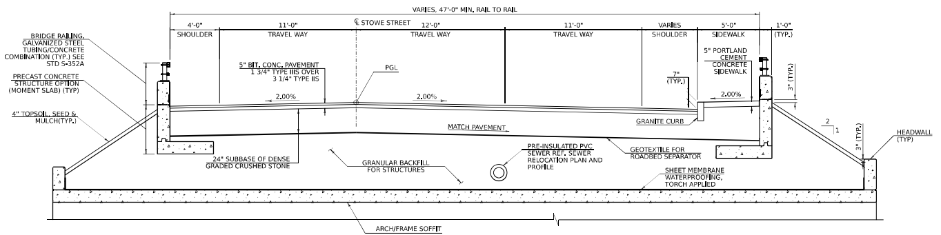
PROPOSED BRIDGE TYPICAL SECTION N.T.S.
