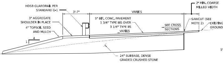
STOWE STREET LEFT TO ROUTE 100 NOT TO SCALE STA. 32+19 - 32+95 LT
