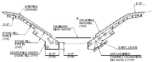
TYPICAL CHANNEL SECTION NOT TO SCALE
