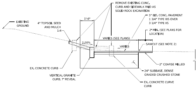
STOWE STREET LT NOT TO SCALE STA. 30+10 - 31+00
